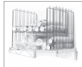
Two 21" tall dividers with one horizontal divider. 8.625" (219mm) space between base and bottom of top shelf.
