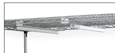
Adjustable Undershelf Slide
