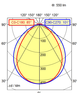
illuminance
