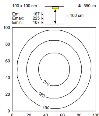
luminous intensity
