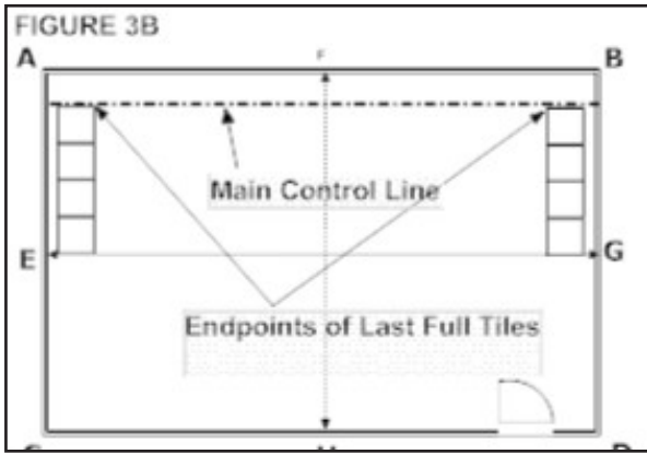
Figure 3B Establish Control Lines
