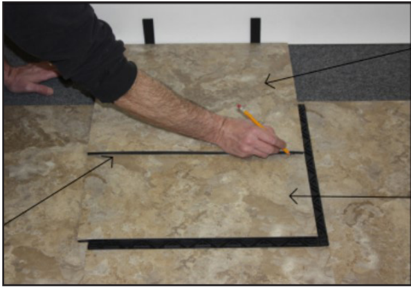
Figure 4 Measuring & Laying Cut Edge Tiles
