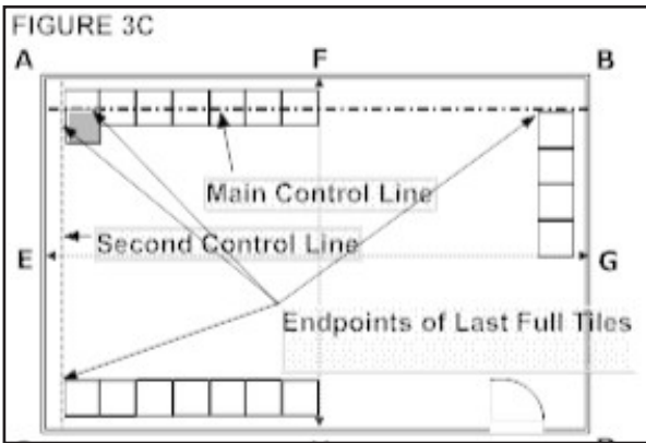
Figure 3C Establish Starting Point
