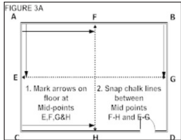
Figure 3A Establishing Midlines & Midpoints
