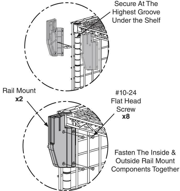
Position Rail Mounts Around The Post
