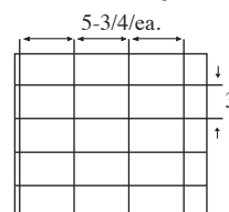
15 Cell Arrangement Max Cell size 5-3/4 x 3-1/2 x 2-1/4" 4 Short Partitions - 4 Long Partitions
