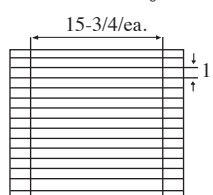
15 Cell Arrangement Max Cell size 15-3/4 x 1 x 2-1/4" 2 Short Partitions - 14 Long Partitions
