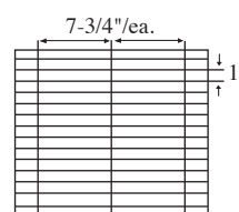
30 Cell Arrangement Max Cell size 7-3/4 x 1 x 2-1/4" 3 Short Partitions - 14 Long Partitions
