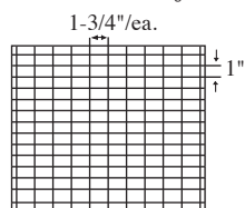
150 Cell Arrangement Max Cell size 1-3/4 x 1 x 2-1/4" 11 Short Partitions - 14 Long Partitions
