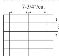
10 Cell Arrangement Max Cell size 7-3/4 x 3-1/2 x 2-1/4" 3 Short Partitions - 4 Long Partitions
