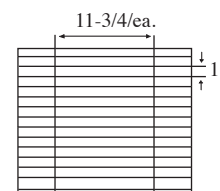
15 Cell Arrangement Max Cell size 11-3/4 x 1 x 2-1/4" 2 Short Partitions - 14 Long Partitions
