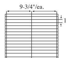
30 Cell Arrangement Max Cell size 9-3/4 x 1 x 2-1/4" 3 Short Partitions - 14 Long Partitions
