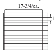
15 Cell Arrangement Max Cell size 17-3/4 x 1 x 2-1/4" 2 Short Partitions - 14 Long Partitions
