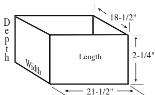
45 Cell Arrangement Max Cell size 5-3/4 x 1 x 2-1/4" 4 Short Partitions - 14 Long Partitions
