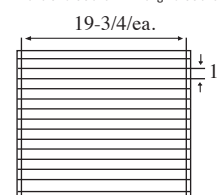
15 Cell Arrangement Max Cell size 19-3/4 x 1 x 2-1/4" 2 Short Partitions - 14 Long Partitions
