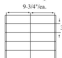
10 Cell Arrangement Max Cell size 9-3/4 x 2-1/4 x 2-1/4" 3 Short Partitions - 4 Long Partitions
