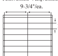
14 Cell Arrangement Max Cell size 9-3/4 x 2-1/4 x 2-1/4" 3 Short Partitions - 7 Long Partitions
