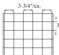
25 Cell Arrangement Max Cell size 3-3/4 x 3-1/2 x 2-1/4" 6 Short Partitions - 14 Long Partitions
