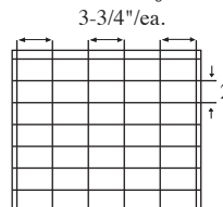
35 Cell Arrangement Max Cell size 3-3/4 x 2-1/4 x 2-1/4" 6 Short Partitions - 7 Long Partitions
