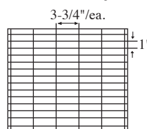
75 Cell Arrangement Max Cell size 3-3/4 x 1 x 2-1/4" 6 Short Partitions - 14 Long Partitions
