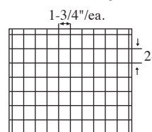
70 Cell Arrangement Max Cell size 1-3/4 x 2-1/4 x 2-1/4" 11 Short Partitions - 7 Long Partitions
