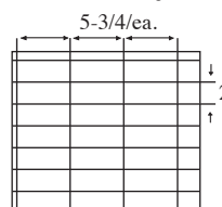
21 Cell Arrangement Max Cell size 5-3/4 x 2-1/4 x 2-1/4" 4 Short Partitions - 7 Long Partitions
