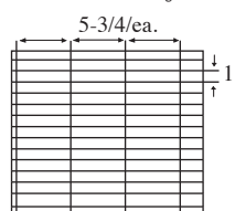
45 Cell Arrangement Max Cell size 5-3/4 x 1 x 2-1/4" 4 Short Partitions - 14 Long Partitions
