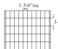
50 Cell Arrangement Max Cell size 1-3/4 x 3-1/2 x 2-1/4" 11 Short Partitions - 4 Long Partitions
